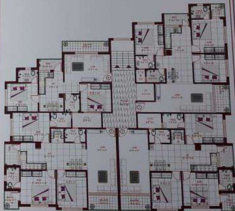
TYPICAL FLOOR
